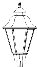
6134RLED H: 38 1/2" W: 21 1/4" EPA: 2.60 Fitter: 3" I.D.
