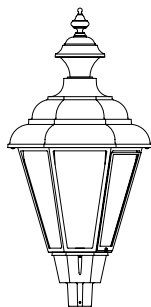
30834RLED H: 42 3/4" W: 20 3/4" EPA: 2.60 Fitter: 3" I.D.
