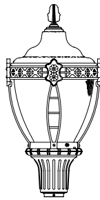
3173LED H: 36" W: 17 1/2" EPA: 2.02 Fitter: 3" I.D.
