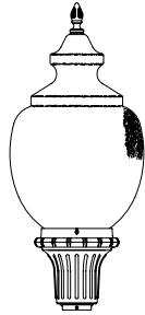
1972LED H: 38" W: 16 1/2" EPA: 2.50 Fitter: 3" I.D.
