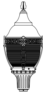
33530LED H: 38 1/2" W: 17" EPA: 2.35 Fitter: 3" I.D.
