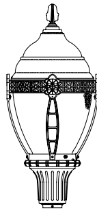
3177LED H: 33 3/4" W: 13 3/4" EPA: 1.35 Fitter: 3" I.D.
