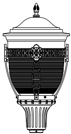
33230LED H: 35 1/4" W: 18 1/8" EPA: 2.15 Fitter: 3" I.D.
