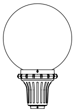
2270LED H: 27" W: 18" EPA: 2.23 Fitter: 3" I.D.
