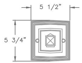
FRONT VIEW OF BRACKET ARM AND WALLPLATE
