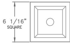
BOTTOM VIEW OF CEILING CANOPY
