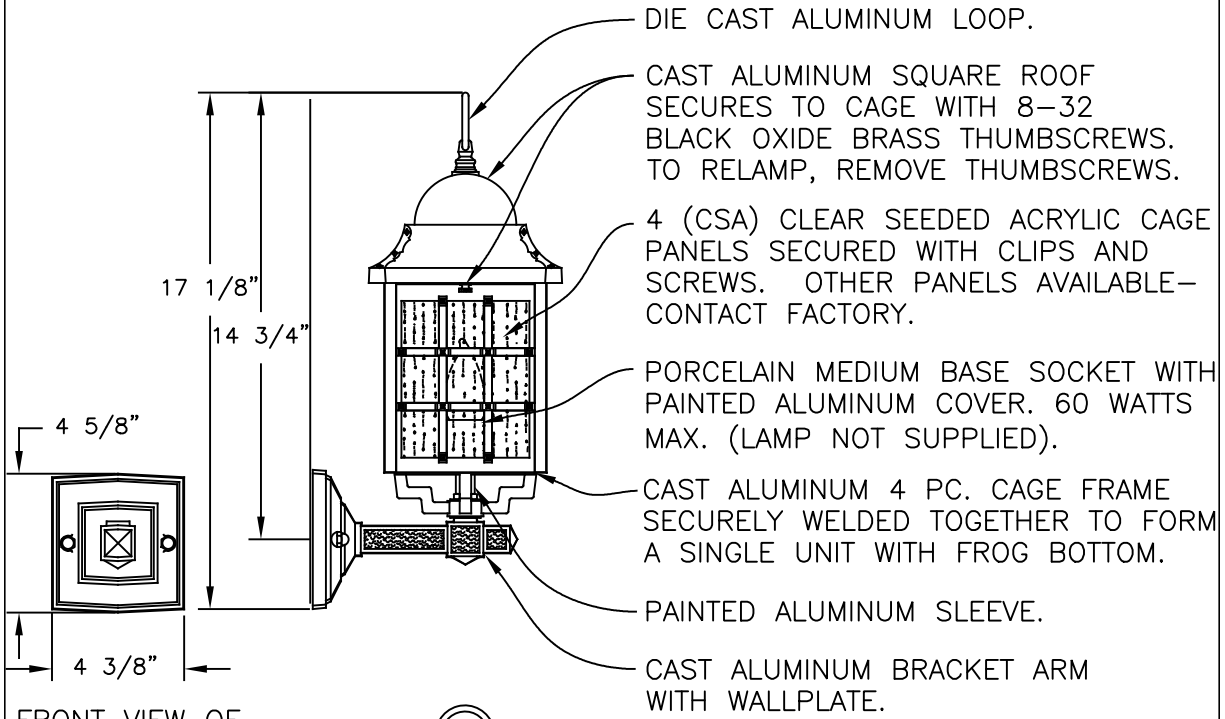
FRONT VIEW OF BRACKET ARM W/WALLPLATE
