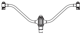
263DB Double Bracket Arm H: 33 7/8" W: 93 1/8"R EPA: 2.00
