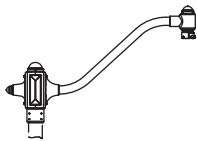
263 Single Bent Bracket Arm H: 33 7/8" W: 55" EPA: 1.30
